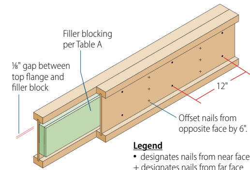
FIGURE A: DOUBLE JOIST CONSTRUCTION
