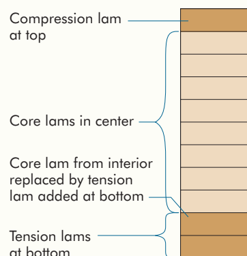
ONE-HOUR FIRE-RATED GLULAM BEAM (Layup for simple span)
