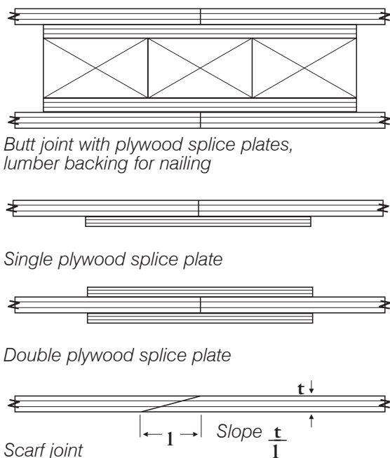
Figure 4. Various Joint Types
