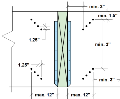
FIGURE 9: 16 NAILS
