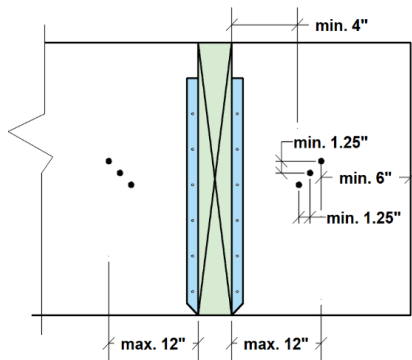
FIGURE 17: 6 WSWH/WS SCREWS
