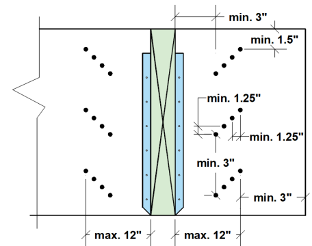
FIGURE 11: 24 NAILS
