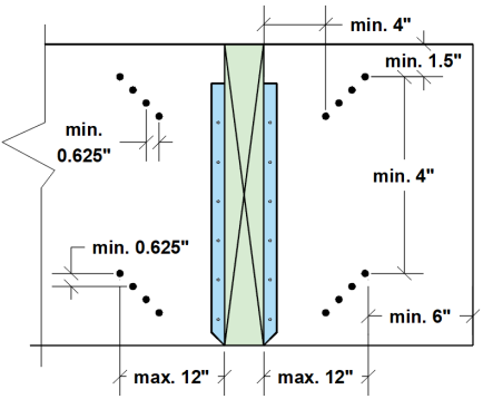
FIGURE 15: 16 SDW SCREWS
