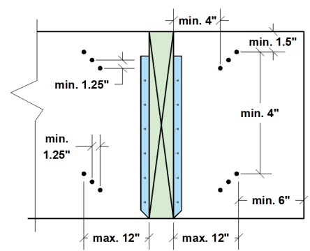
FIGURE 19: 12 WSWH/WS SCREWS
