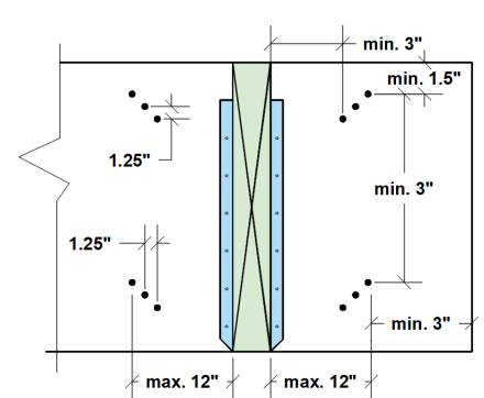
FIGURE 11: 24 NAILS
