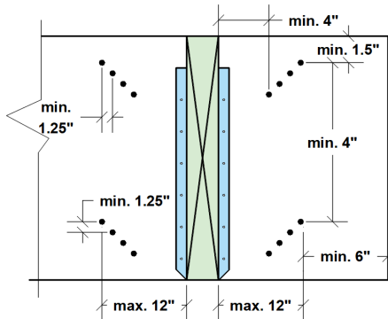
FIGURE 20: 16 WSWH/WS SCREWS
