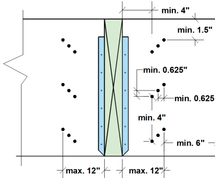
FIGURE 16: 18 SDW SCREWS
