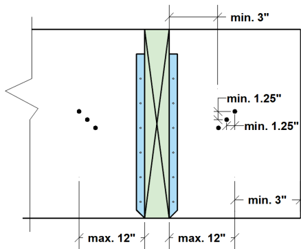
FIGURE 9: 16 NAILS
