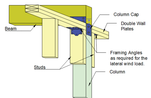
Detail 19: Beam on Column
