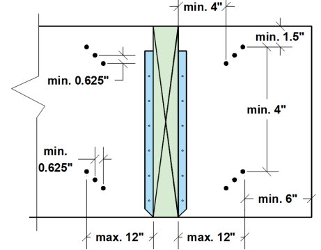
FIGURE 14: 12 SDW SCREWS
